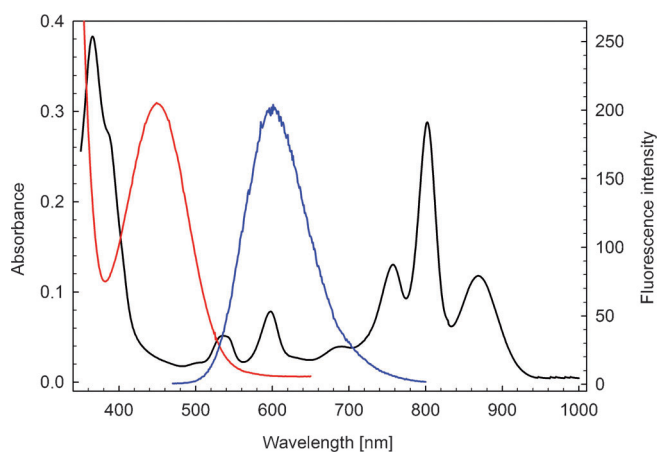
Figure 2. Absorption spectra of RC (—) and AE (—). Fluorescence spectrum of AE (—). RC (1 μM), AE (4 μM) in Tris (20 mM), EDTA (1 mM), TX-100 (0.03 %, pH 8; TTE buffer). AE spectra are multiplied by a factor of two. The spectrum of the RC shows several peaks, which arise from the D (860 nm), the monomer Bchl (801 nm), and from the BΦ (765 nm).
